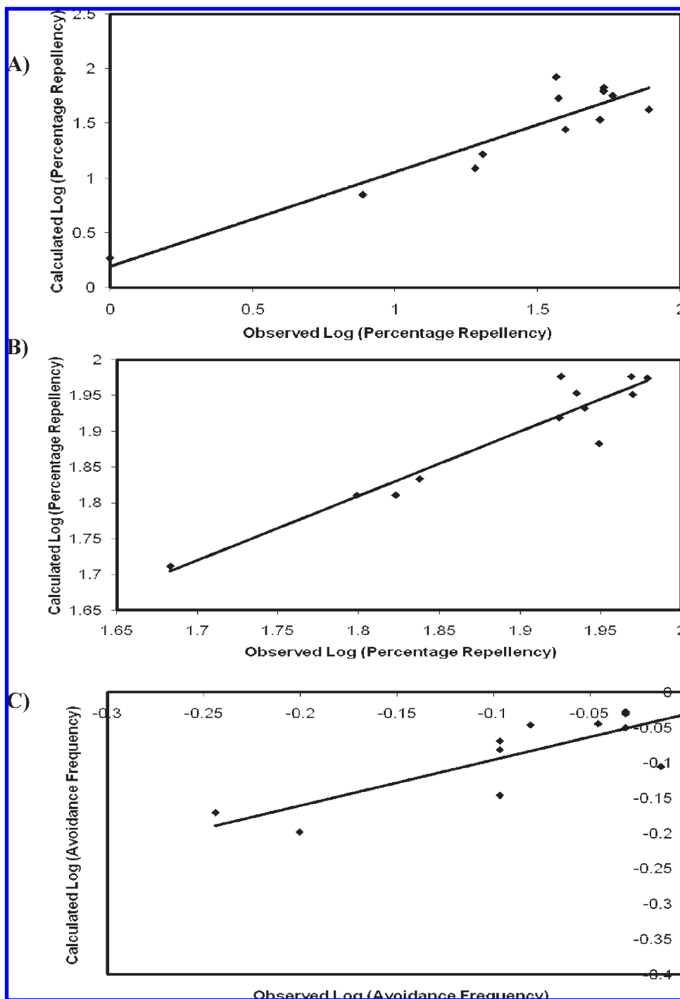
Figure 2. Calculated versus observed spatial and contact repellency values shown for three of the five sesquiterpene repellency models: (A) spatial 15 min; (B) spatial 180 min; (C) contact repellency.
