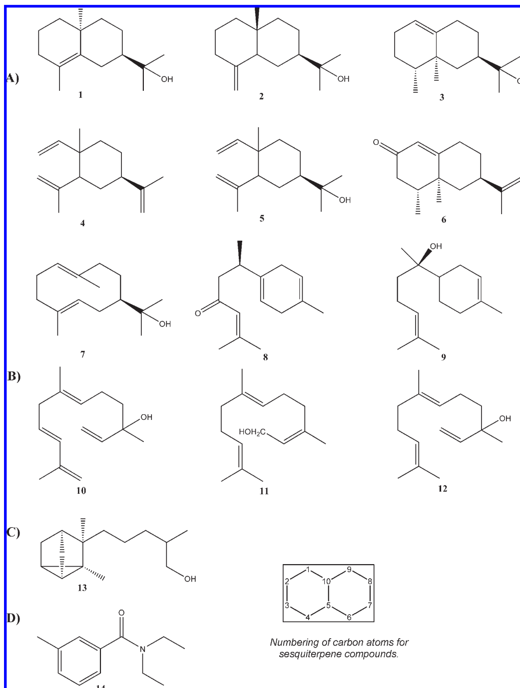
Figure 1. Structures of sesquiterpenes and DEET ( N,N -diethyl- m -methylbenzamide): (A) eudesmane, elemene, eremophilane, bisabone, and germacrane compounds; (B) acyclic; (C) bridged system; (D) DEET.
